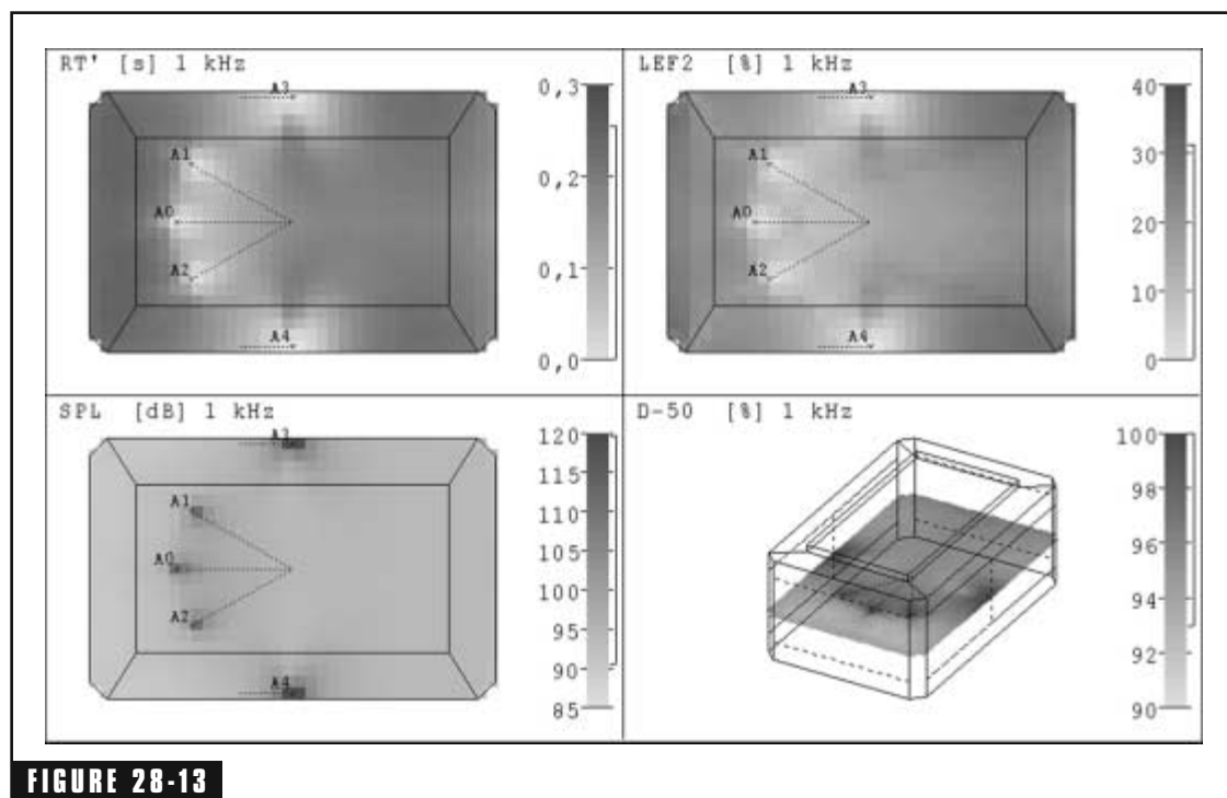
FIGURE 28-13 The perceived reverberation time RT' , lateral energy fraction LEF2, the sound-pressure level SPL, and the energy ratio D50 are mapped at 1 kHz across the room with a THX configuration of left/center/right and dipole surrounds.
