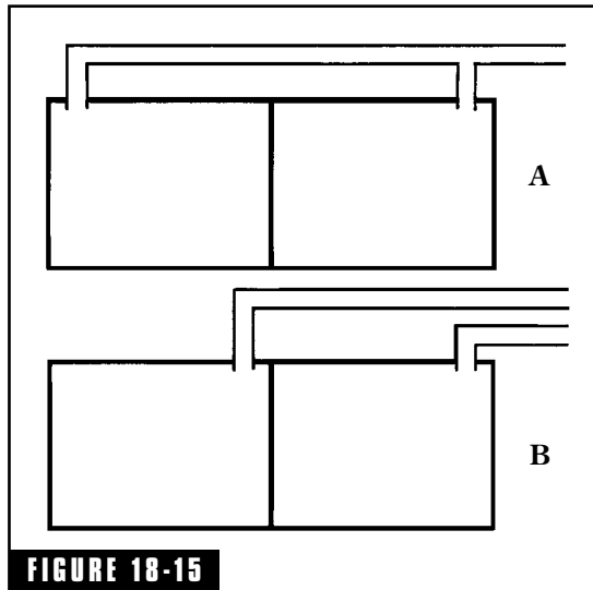
FIGURE 18-15 Two possible solutions to the problems of Fig. 18-14. (A) Separate grilles as far as possible. (B) Feed each room with a separate duct. Both approaches increase duct path length and thus duct attenuation.
