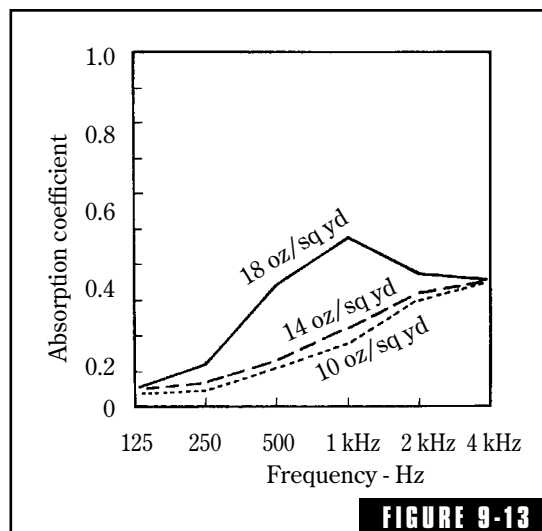
FIGURE 9-13 The sound absorption of velour hung straight for three different weights of fabric. (After Beranek. 18 )
