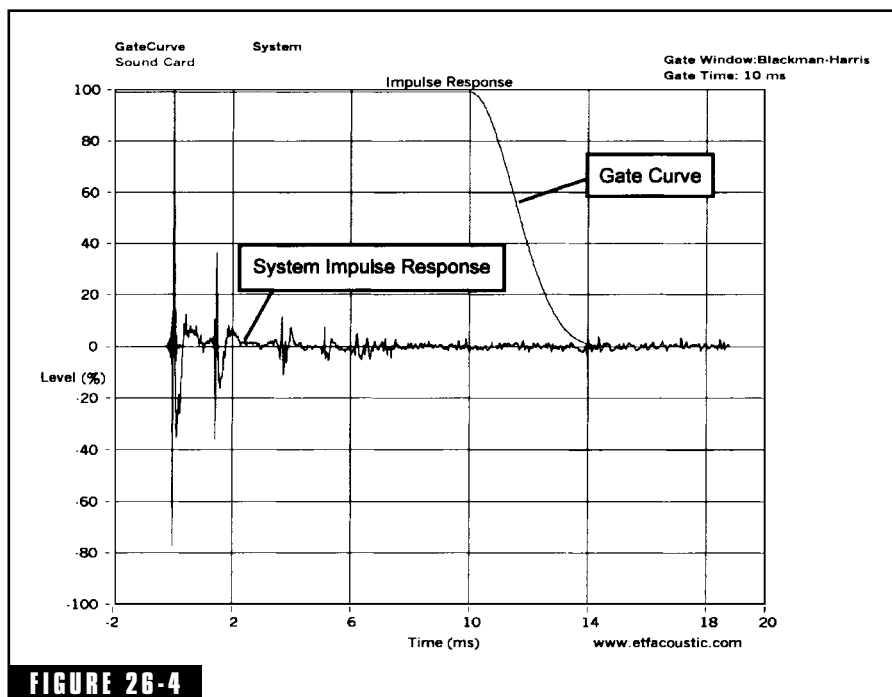
Impulse response of a loudspeaker measured at a distance of 1 m, with a single reflecting surface nearby. (Courtesy of Doug Plumb, AcoustiSoft.)
