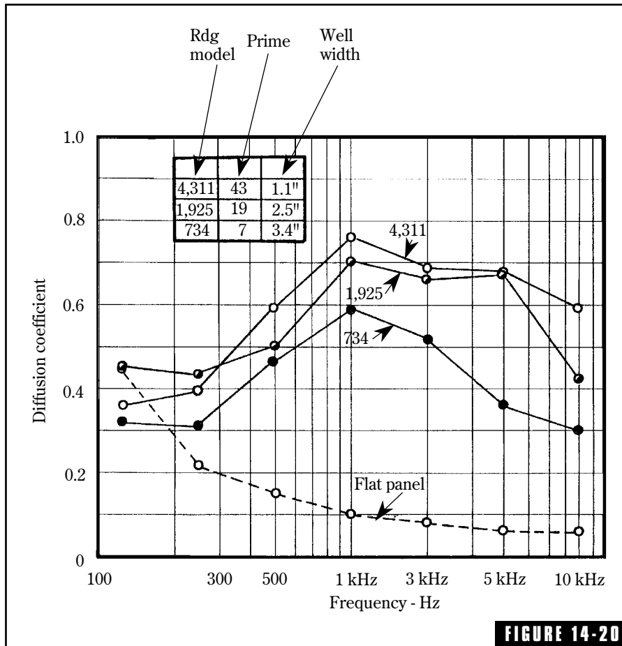
FIGURE 14-20 Comparison of the variation of diffusion coefficient with frequency of three RPG™ difusors and a flat panel. Peter D'Antonio, RPG Diffusor Systems, Inc.
