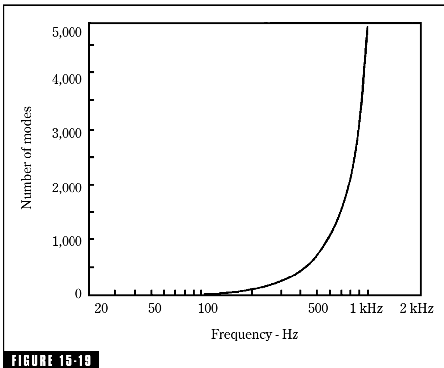
The number of modal frequencies increases dramatically with frequency.
