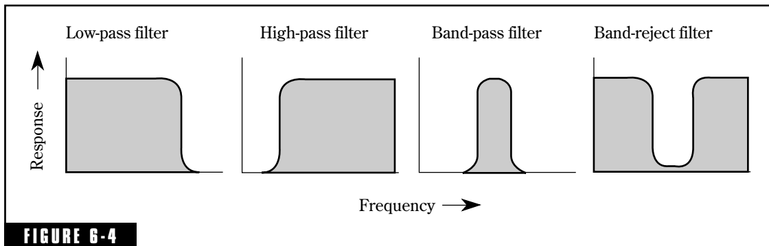
Basic response shapes for the low-pass, high-pass, band-pass, and band-reject filters.
