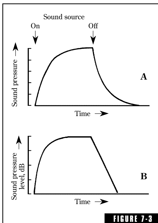
FIGURE 7-3 The growth and decay of sound in a room. (A) Vertical scale in linear sound pressure units. (B) The vertical scale in logarithmic units (decibels).
