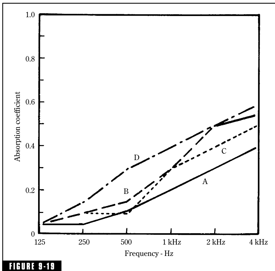
FIGURE 9-19 Carpet absorption coefficients from a commonly used table. (A) \frac{1}{8} " pile height. (B) \frac{1}{4} " pile height. (C) \frac{3}{16} " combined pile and foam. (D) \frac{5}{16} " combined pile and foam. Compare these graphs with those of Figs. 9-16 and 9-17. 6
