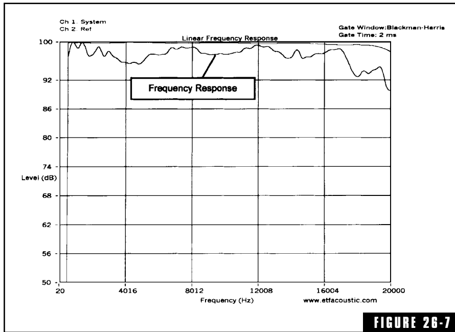
Frequency response of a loudspeaker measured at a distance of 1 m, with minimal reflections. (Courtesy of Doug Plumb, AcustiSoft.)
