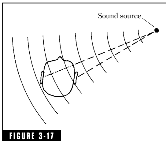
Our binaural directional sense is dependent in part on the difference in intensity and phase of the sound falling on two ears.
