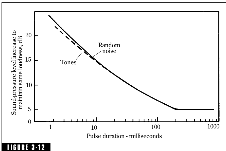
FIGURE 3-12 Short pulses of tones or noise are less audible than longer pulses as these graphs indicate. The discontinuity of the 100- to 200-msec region is related to the integrating time of the ear.
