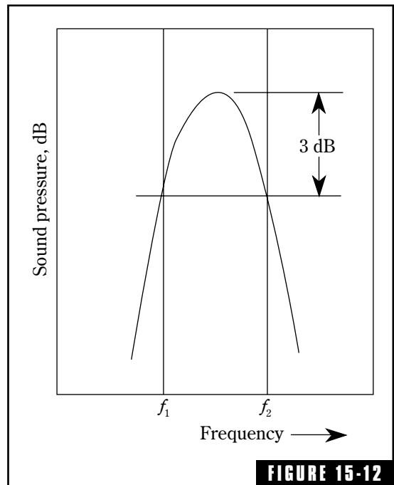
FIGURE 15-12 Each mode has a finite bandwidth. The more absorbent the room, the greater the bandwidth. As measured at the customary -3-dB points, the modal bandwidth of a recording studio is near 5 Hz.
