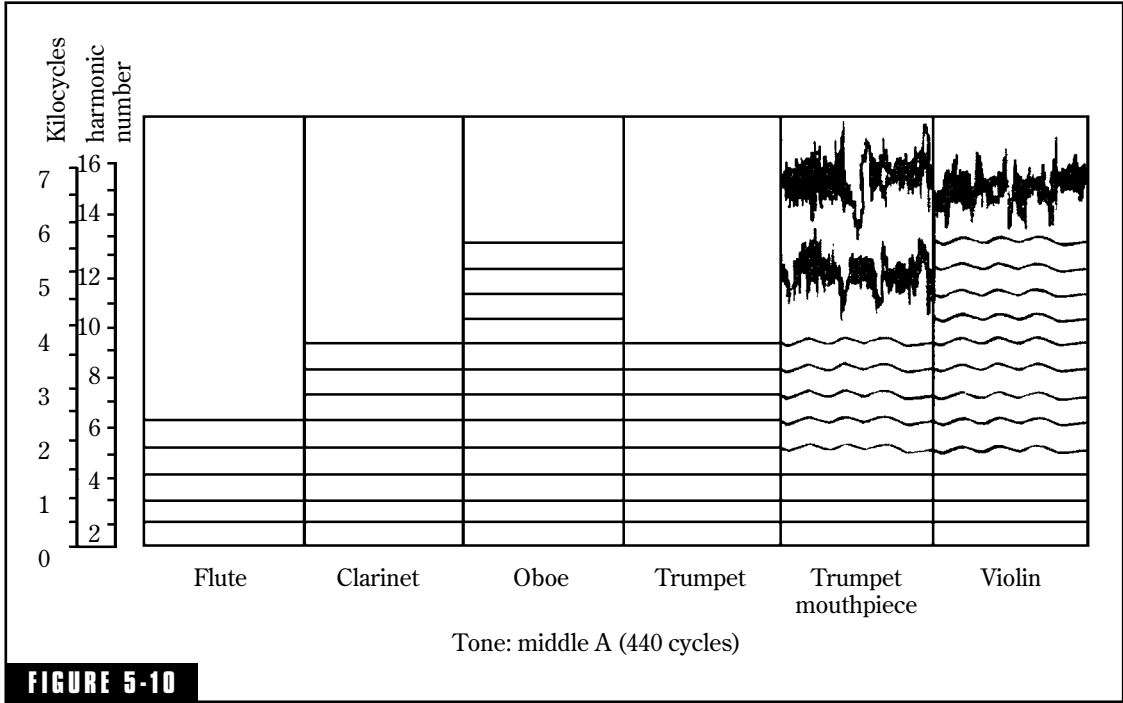
FIGURE 5-10 Spectrogram comparison of the harmonic content of woodwind instruments and the violin as middle A (440 Hz) is played. The differences displayed account for the difference in timbre of the different instruments. AT&T Bell Laboratories.
