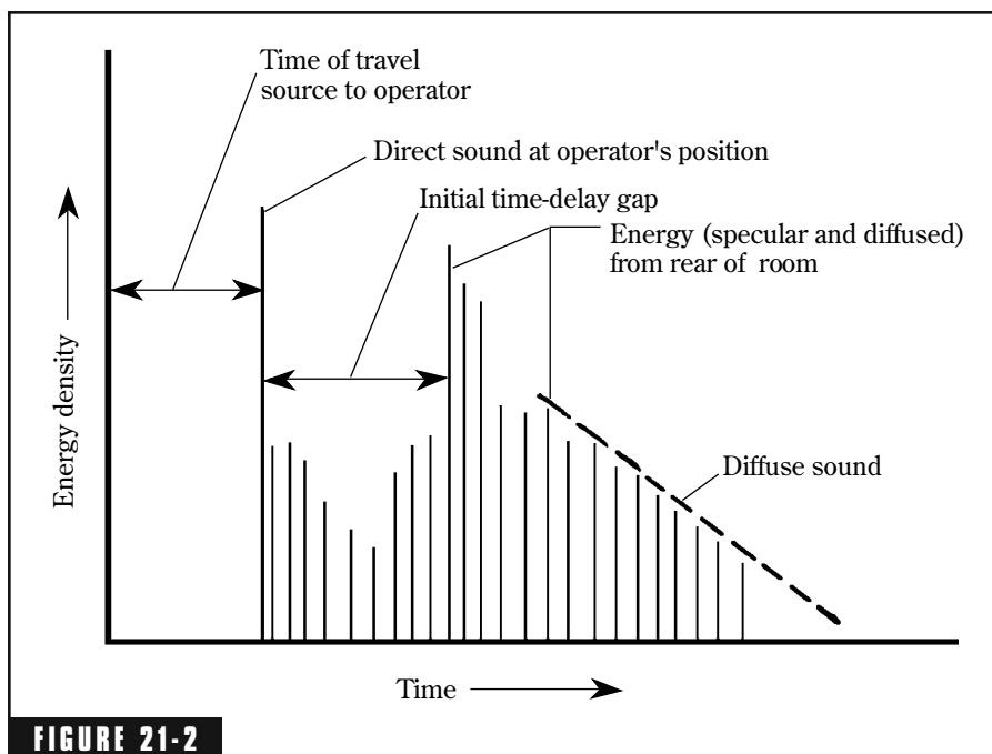
FIGURE 21-2 The definition of the initial time-delay gap for a control room.
