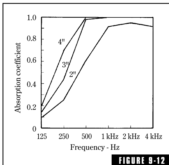
FIGURE 9-12 Absorption coefficients of Sonex contoured foam of various thicknesses. 4
