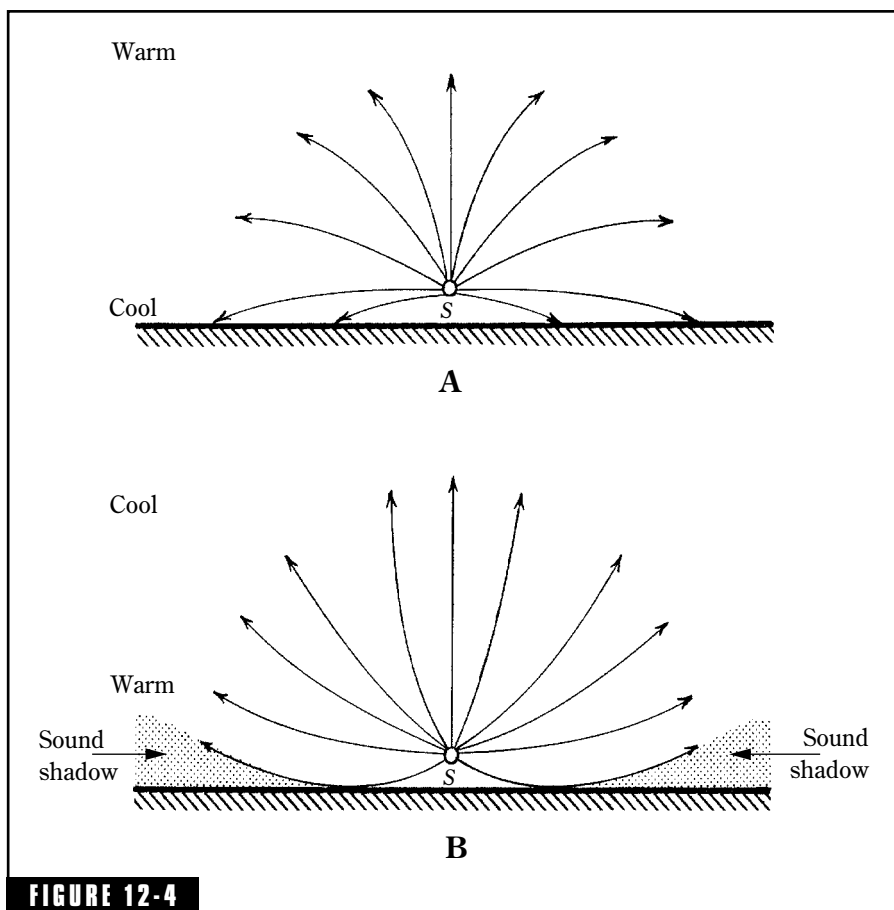
Comprehensive illustration of refraction of sound from source S; (A) cool air near the ground and warmer air above, (B) warm air near the ground and cooler air above. In (B) note that sound shadow areas result from the upward refraction.
