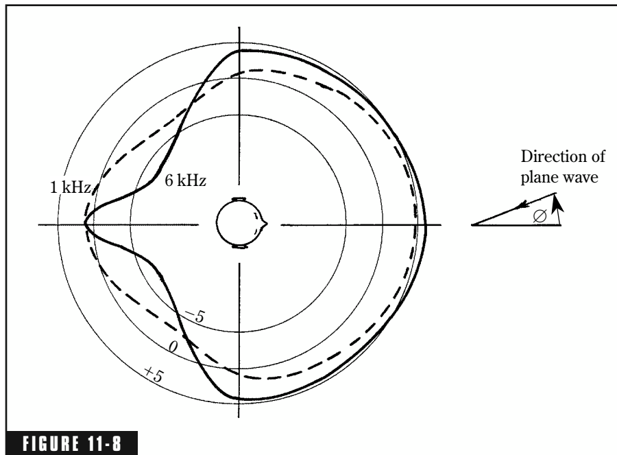
FIGURE 11-8 Diffraction around a solid sphere about the size of a human head. For sound in the 1-6 kHz range, sound pressure is generally increased in the front hemisphere and generally reduced in the rear. (After Muller, Black and Davis, as reported by Olson. 2 )
