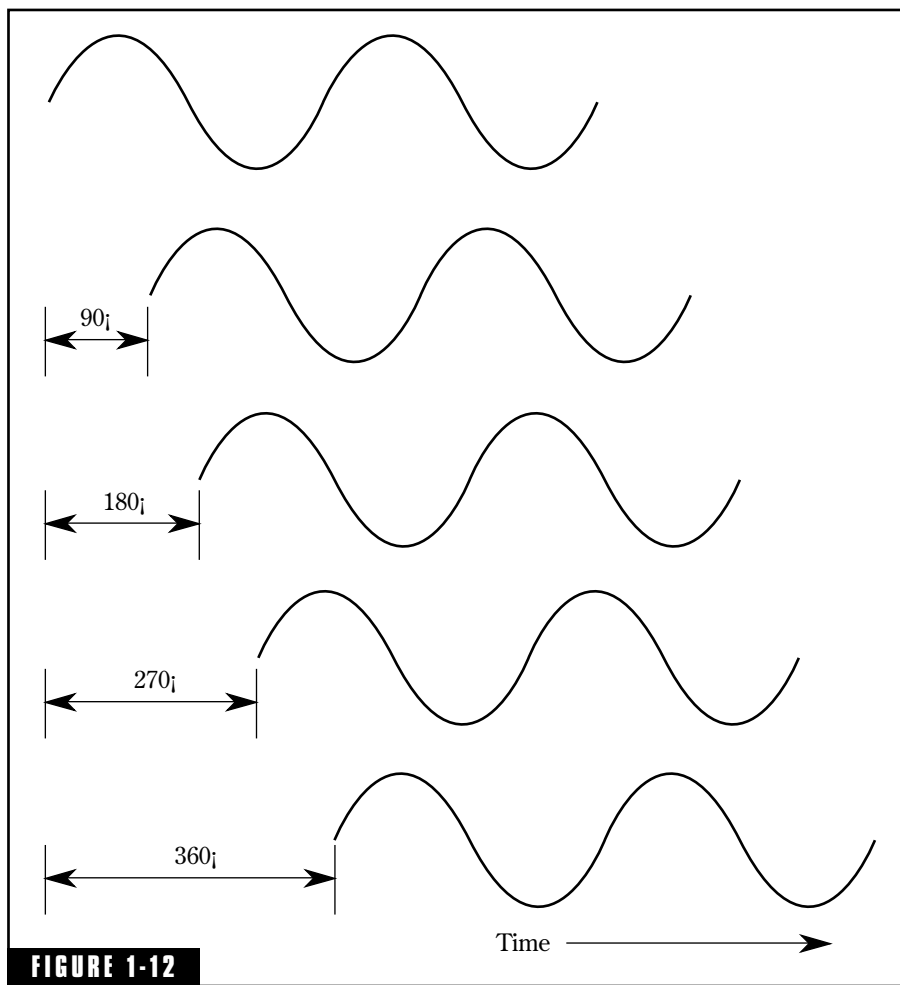
FIGURE 1-12 Illustration of the phase relationships between waves with the same amplitude and frequency. A rotation of 360^\circ is analogous to one complete sine cycle.
