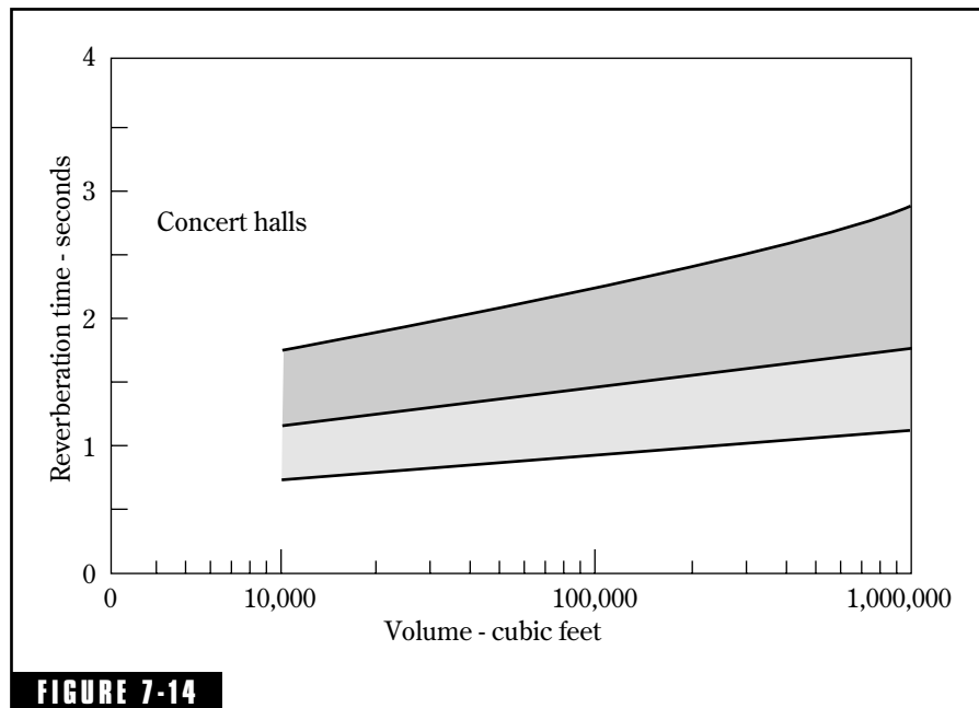
FIGURE 7-14 “Optimum” reverberation time for concert halls. Symphony orchestras are near the top of the shaded areas; lighter music is lower. The lower shaded area applies to opera and chamber music.
