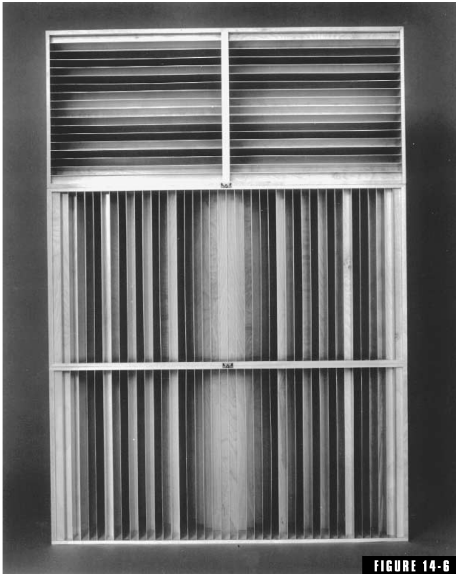
FIGURE 14-6 A cluster of commercial quadratic-residue diffusers. Below are two QRD-4311™ diffusing modules with a single QRD-1911™ mounted above. The hemidisc of diffusion for the lower unit is horizontal, that of the upper unit is vertical. Peter D'Antonio, RPG Diffusor System, Inc. and the Audio Engineering Society, Inc.
