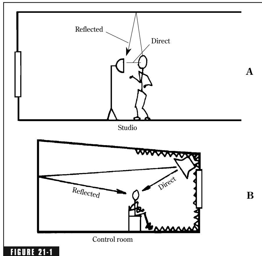
FIGURE 21-1 The wider time-delay gap of a live-end-dead-end control room avoids masking that of the studio. After Davis. 2
