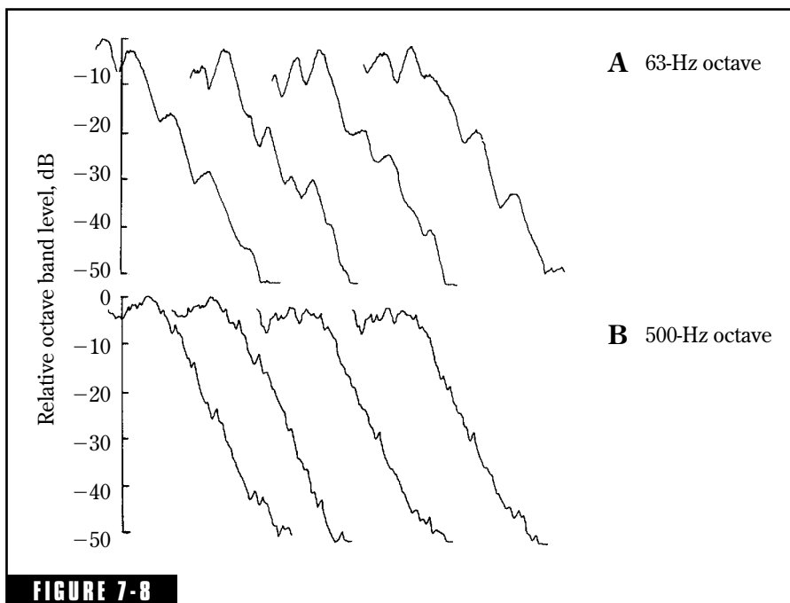
FIGURE 7-8 Actual decays of random noise recorded in a small studio having a volume of 2,921 cu ft; (A) Four successive 63-Hz octave decays recorded under identical conditions. (B) Four successive 500-Hz octave decays also recorded under identical conditions. The differences noted result from the differences in random-noise excitation the instant the switch is opened to start the decay.
