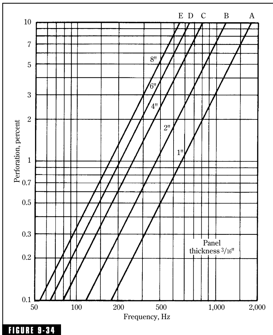
FIGURE 9-34 A graphic presentation of Eq. 9-4 relating percent perforation of perforated panels, the depth of air space, and the frequency of resonance. The graphs are for a panel of \frac{3}{16} inch thickness. (See also Fig. 9-21.) (A) For 1 inch furring lumber. The lines are drawn to correspond to furring lumber which is furnished, e.g., the line for 8 inch is actually 7\frac{3}{4} air-space. (B) For 2 inch furring lumber. (C) For 4 inch furring lumber. (D) For 6 inch furring lumber. (E) For 8 inch furring lumber.
