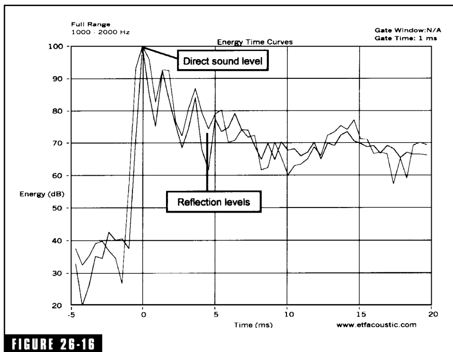
Energy-time curve of a loudspeaker measured at 1 m distance with one or two high-level reflections. (Courtesy of Doug Plumb, AcoustiSoft.)
