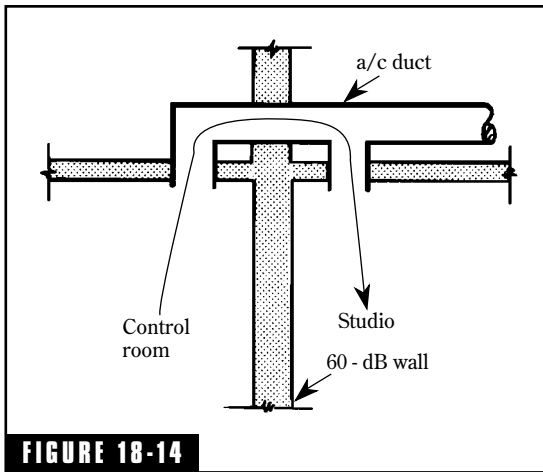
FIGURE 18-14 An expensive, high-transmission-loss wall can be bypassed by sound traveling over a short duct path from grille to grille.
